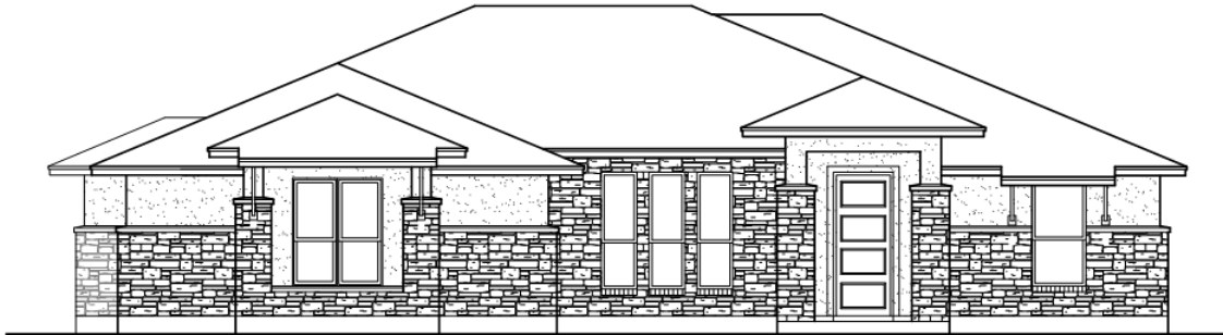
Front Elevation "C"
